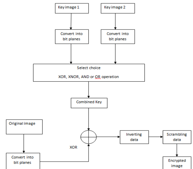
Fig.1 Proposed block diagram for Bitplane Crypt algorithm
